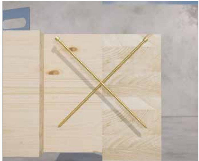
ESCRFT screws in glulam cross pair application.
