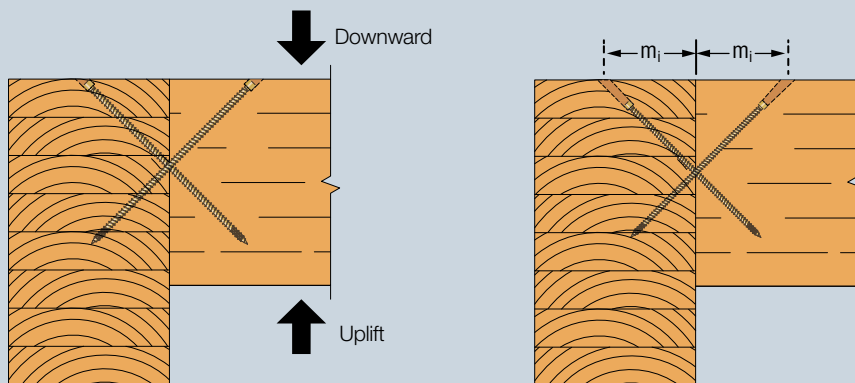
Vertical Load
