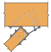
LSSU Installation
