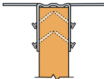
LSSU Installation
