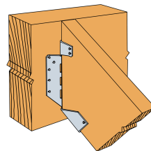
Sloped connection.
