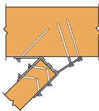
LSSU Installation
