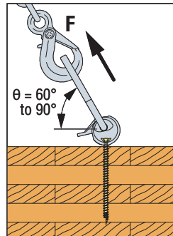
3. Attach rigging to MTLD and lift
