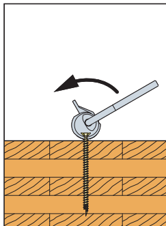
2. Attach MTLD to screw
