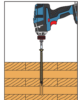
5. Remove screw or drive flush with surface
